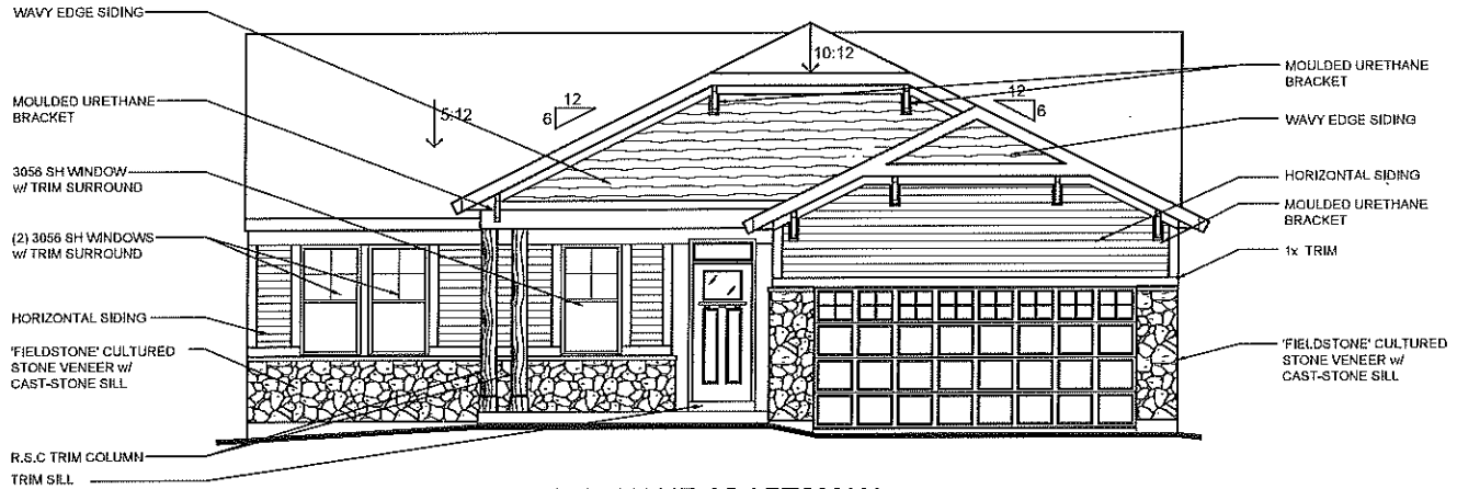
HILLSTONE CRAFTSMAN SHOWN W/ CULTURED STONE VENEER (AVAILABLE w/ LOW STONE SIDES)
