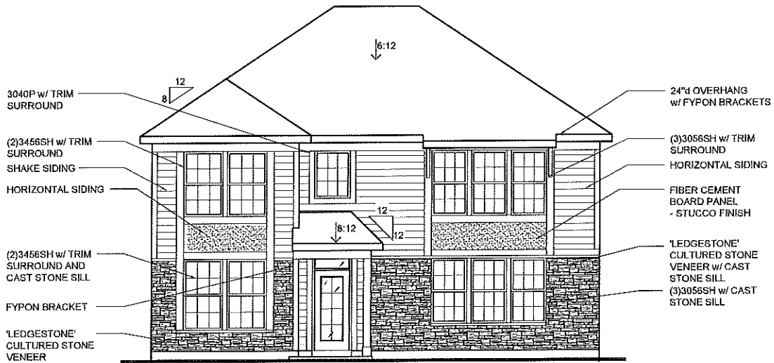
OPT. SIDE ENTRY (AVAILABLE w/ LOW STONE SIDES AND REAR)
