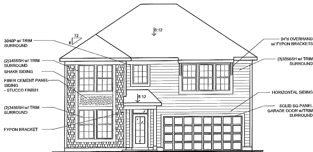
FRONT ENTRY w/ INCLUDED SIDING
