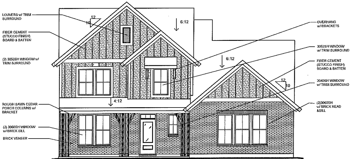
OPT. SIDE ENTRY (AVAILABLE w/ LOW OR HIGH BRICK SIDES & REAR)
