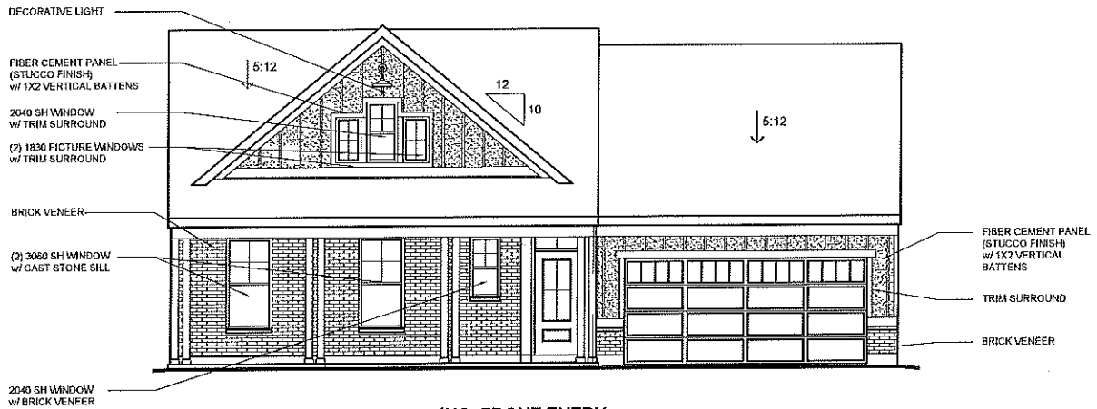
INC. FRONT ENTRY (AVAILABLE w/ LOW OR HIGH BRICK SIDES AND REAR)
