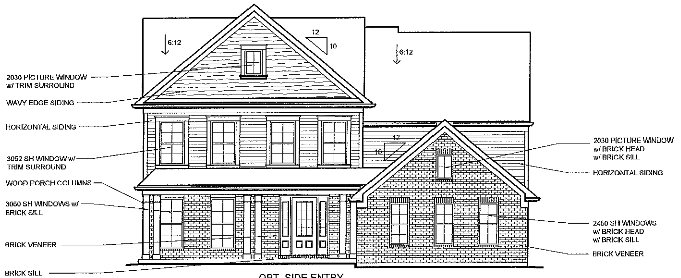
OPT. SIDE ENTRY (AVAILABLE w/ LOW OR HIGH BRICK SIDES AND REAR)
