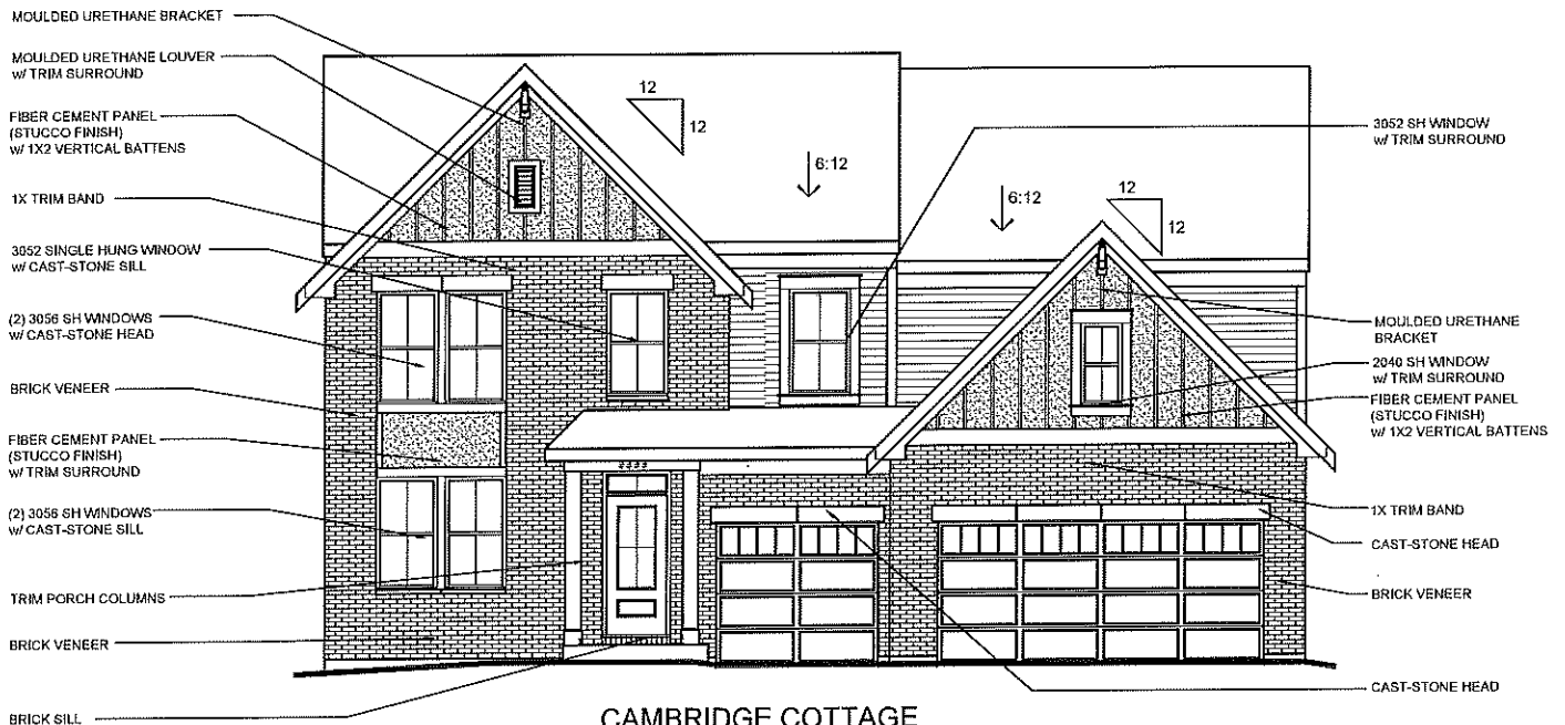
CAMBRIDGE COTTAGE w/ OPT. BRICK VENEER w/ OPT. THREE-CAR INTEGRATED FRONT ENTRY GARAGE AVAILABLE w/ LOW OR HIGH BRICK SIDES
