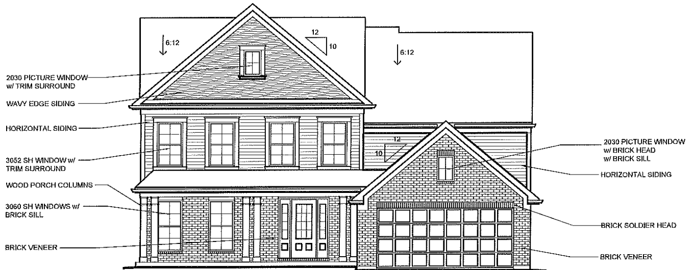
INC. FRONT ENTRY (AVAILABLE w/ LOW OR HIGH BRICK SIDES AND REAR)
