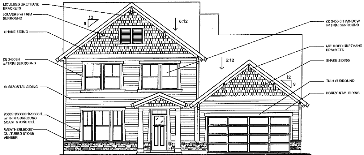
INC. FRONT ENTRY (AVAILABLE w/ LOW STONE SIDES & REAR)
