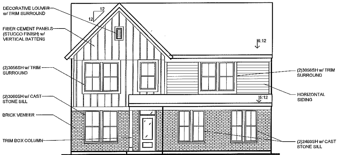
OPT. SIDE ENTRY w/ OPT. BRICK VENEER (AVAILABLE w/ LOW or HIGH BRICK SIDES AND REAR)
