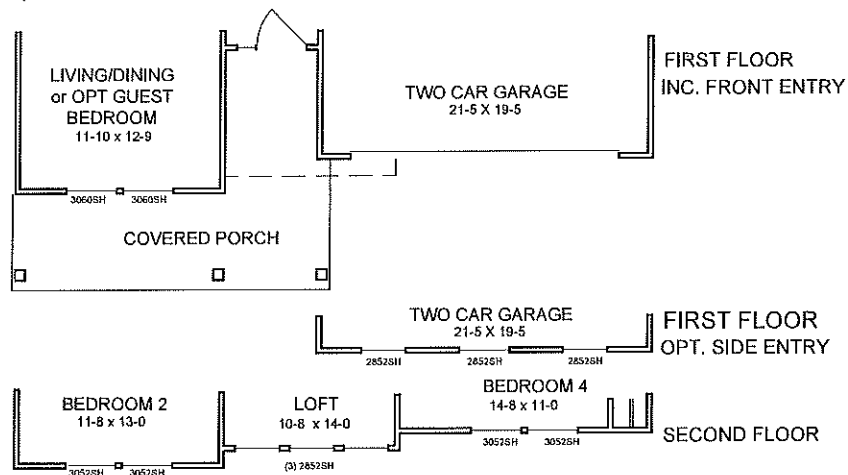
OPT. SIDE ENTRY (AVAILABLE w/ LOW OR HIGH BRICK SIDES AND REAR)
