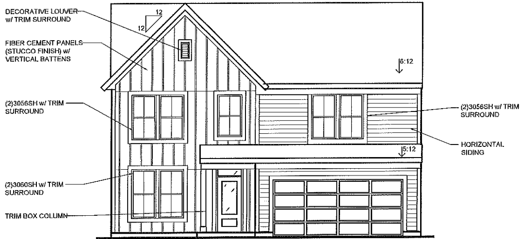
FRONT ENTRY w/ INCLUDED SIDING
