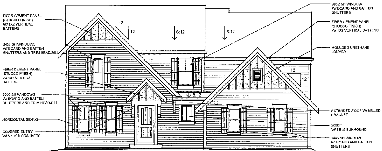
CAMBRIDGE COTTAGE w/ COVERED ENTRY SHOWN w/ OPT. SIDE ENTRY GARAGE
