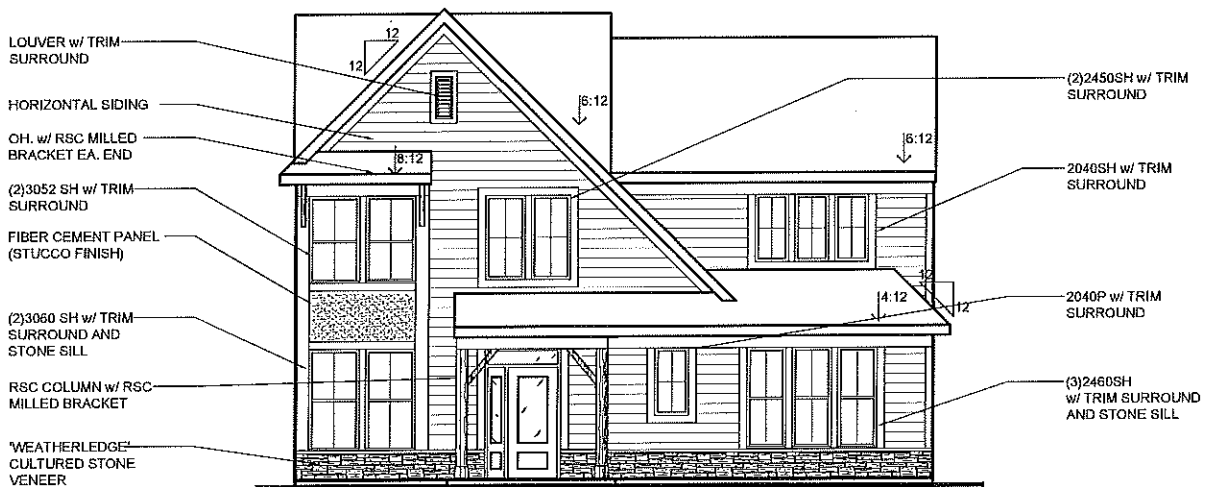
OPT. SIDE ENTRY w/ OPT. CULTURED STONE VENEER (AVAILABLE w/ LOW STONE SIDES AND REAR)
