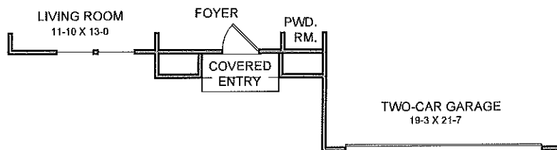
FIRST FLOOR
