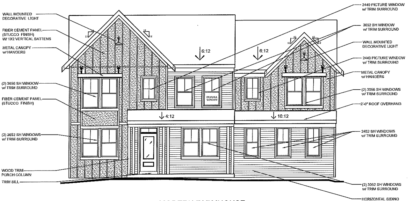
MODERN FARMHOUSE w/ INCL. FRONT PORCH w/ OPT. SIDE ENTRY GARAGE
