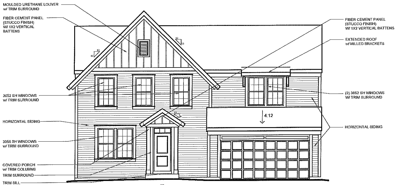
CAMBRIDGE COTTAGE w/ OPT. PORCH
