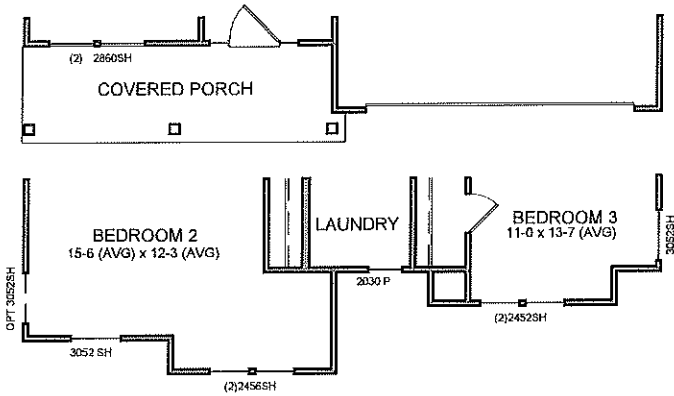
OPT. SIDE ENTRY w/ OPT BRICK VENEER (AVAILABLE w/ LOW OR HIGH BRICK SIDES AND REAR)
