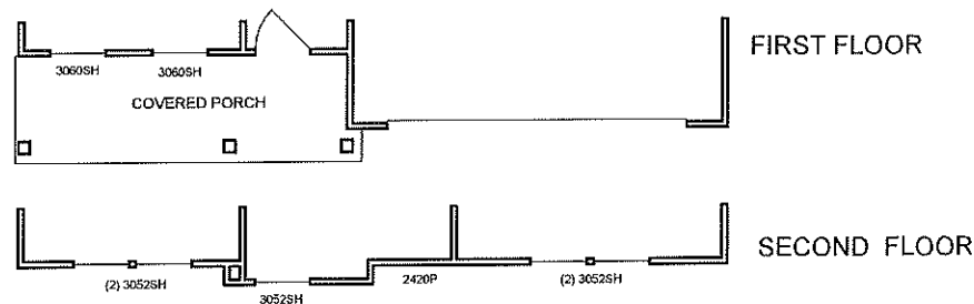
OPT. SIDE ENTRY w/ OPT BRICK VENEER (AVAILABLE w/ LOW or HIGH BRICK SIDES AND REAR)
