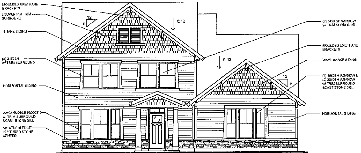
OPT. SIDE ENTRY (AVAILABLE w/ LOW STONE SIDES & REAR)
