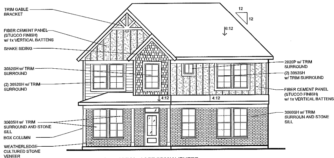
OPT. SIDE ENTRY w/ OPT BRICK VENEER (AVAILABLE w/ LOW or HIGH BRICK SIDES AND REAR)
