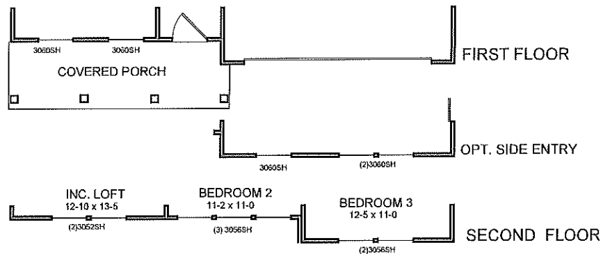
OPT. SIDE ENTRY (AVAILABLE w/ LOW OR HIGH BRICK SIDES AND REAR)
