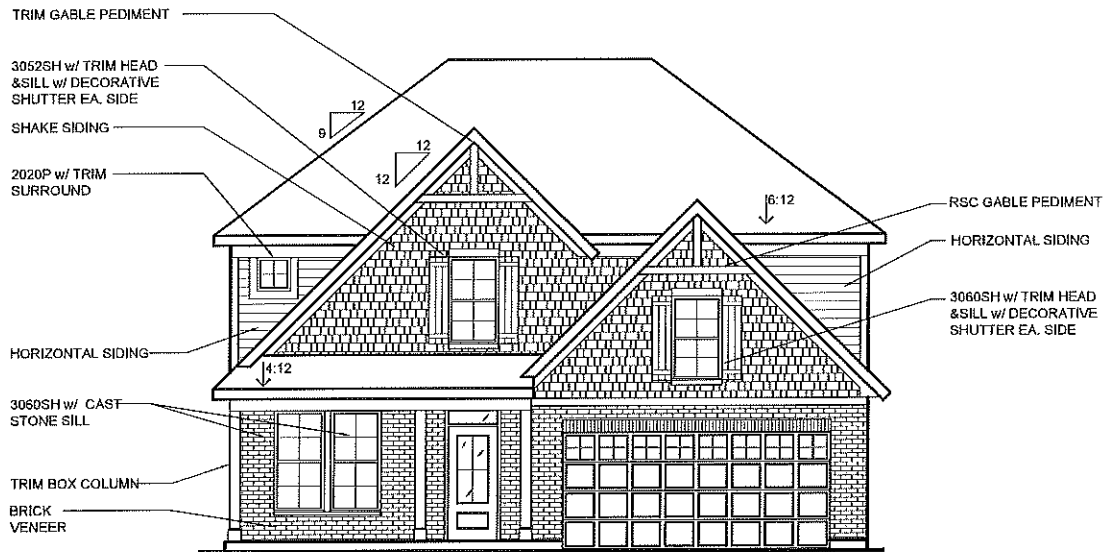
FRONT ENTRY w/OPT. BRICK VENEER (AVAILABLE w/ LOW AND HIGH BRICK SIDES AND REAR)
