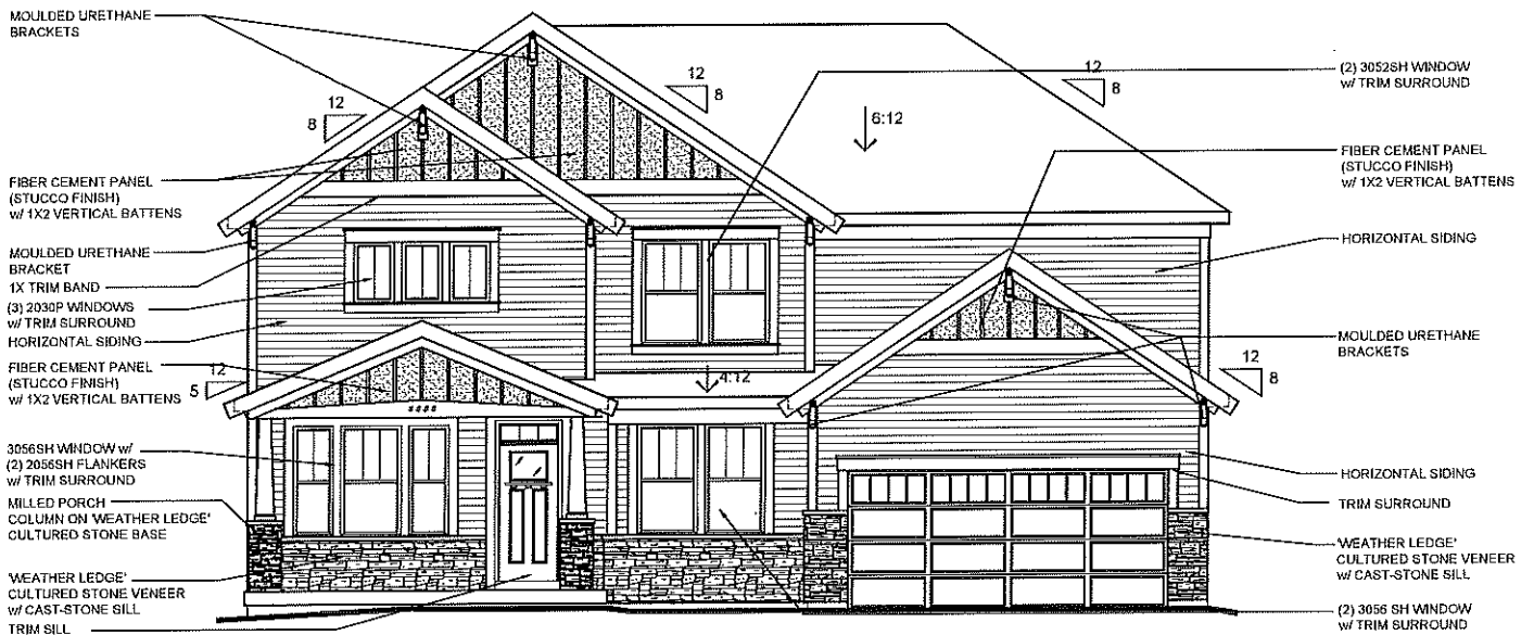
PACIFIC CRAFTSMAN w/ OPT. CULTURED STONE VENEER AVAILABLE w/ LOW STONE SIDES
