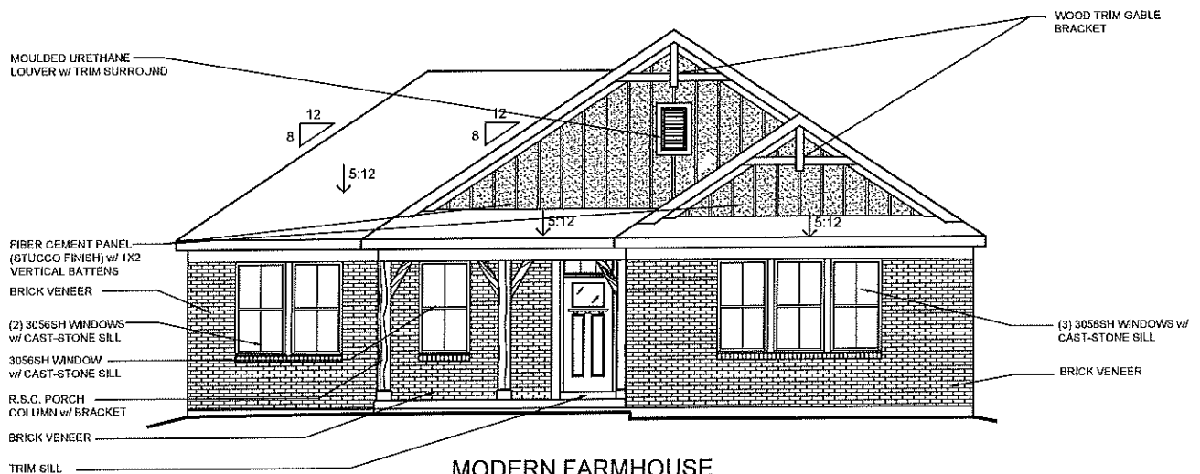
MODERN FARMHOUSE SHOWN w/ OPT. SIDE ENTRY GARAGE SHOWN w/ OPT. BRICK VENEER (AVAILABLE w/ LOW OR HIGH BRICK SIDES)
