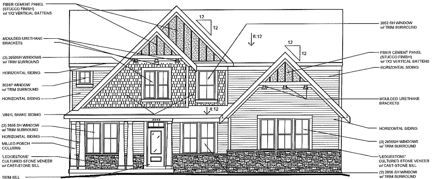
COASTAL CLASSIC w/ OPT. CULTURED STONE VENEER SHOWN w/ OPT. SIDE ENTRY GARAGE AVAILABLE w/ LOW STONE SIDES
