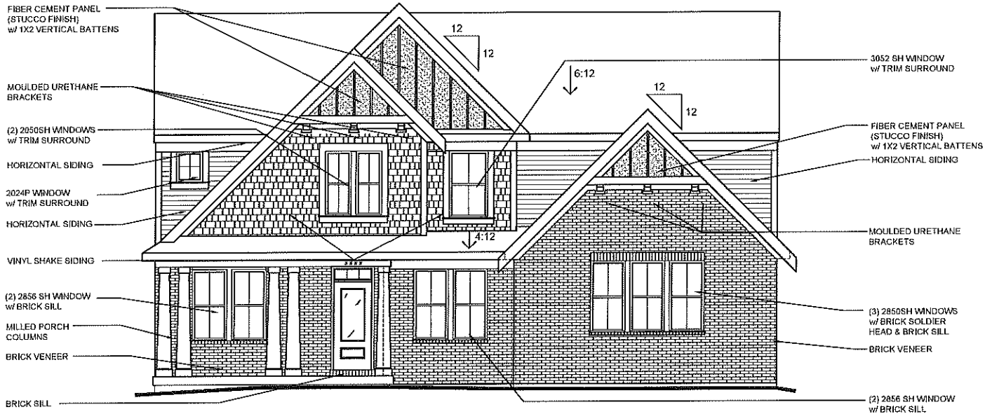
COASTAL CLASSIC SHOWN w/ OPT. SIDE ENTRY GARAGE AVAILABLE w/ LOW OR HIGH BRICK SIDES
