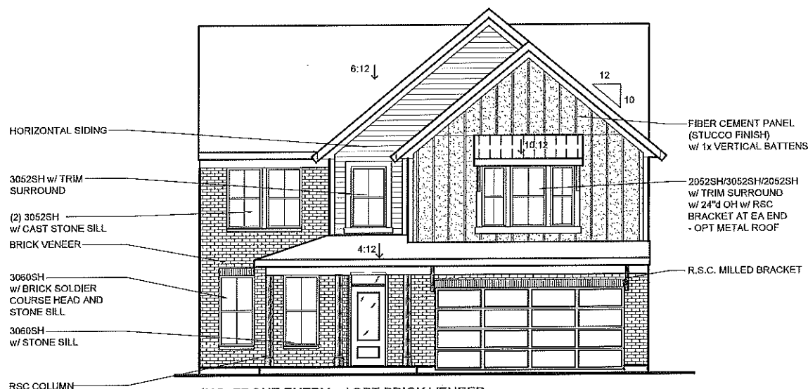
INC. FRONT ENTRY w/ OPT BRICK VENEER (AVAILABLE w/ LOW or HIGH BRICK SIDES AND REAR)
