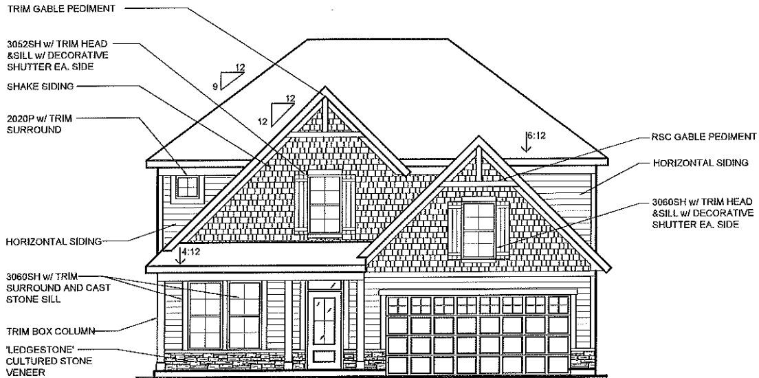
FRONT ENTRY w/OPT. CULTURED STONE VENEER (AVAILABLE w/ LOW STONE SIDES AND REAR)
