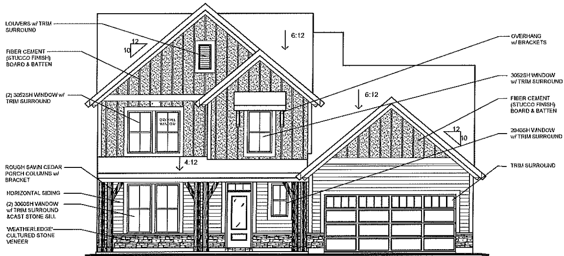
INC. FRONT ENTRY (AVAILABLE w/ LOW STONE SIDES & REAR)
