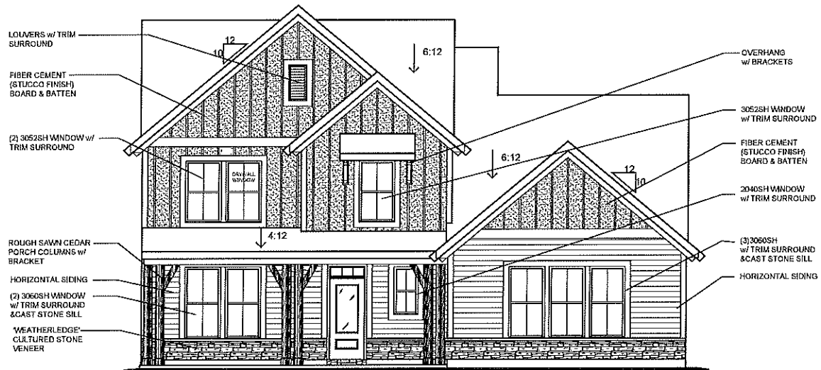
OPT. SIDE ENTRY (AVAILABLE w/ LOW STONE SIDES & REAR)
