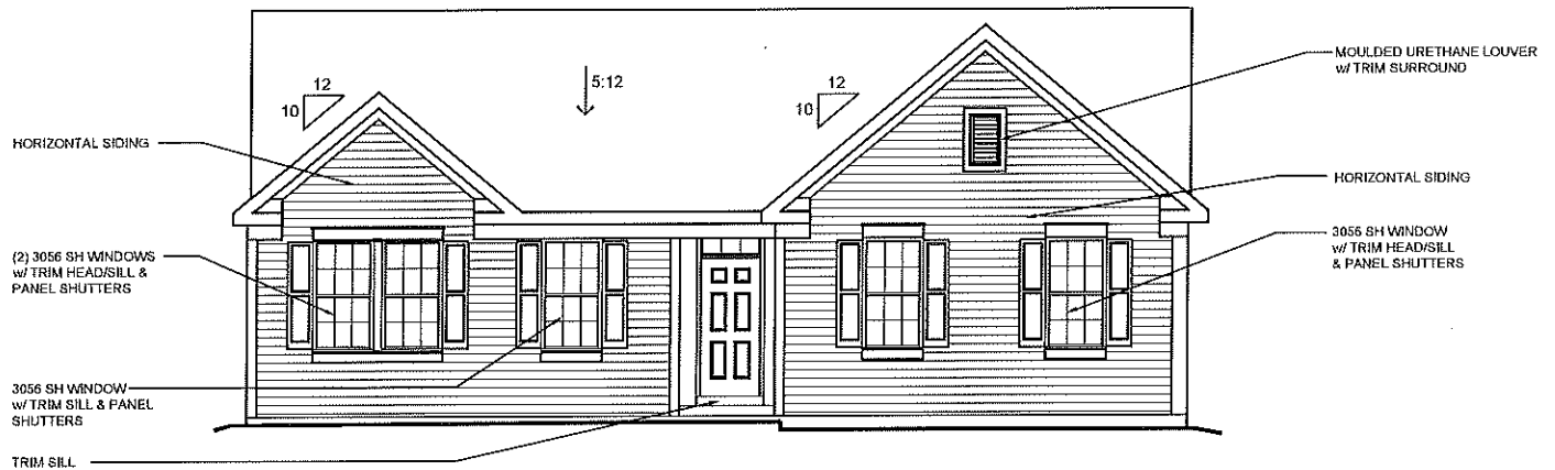
AMERICAN CLASSIC SHOWN w/ OPT. SIDE ENTRY GARAGE
