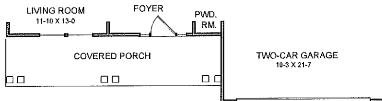
FIRST FLOOR
