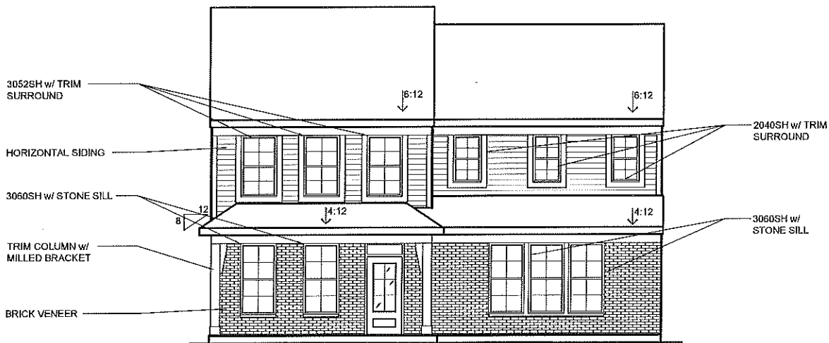
OPT. SIDE ENTRY w/ OPT. BRICK VENEER (AVAILABLE w/ LOW or HIGH BRICK SIDES AND REAR)
