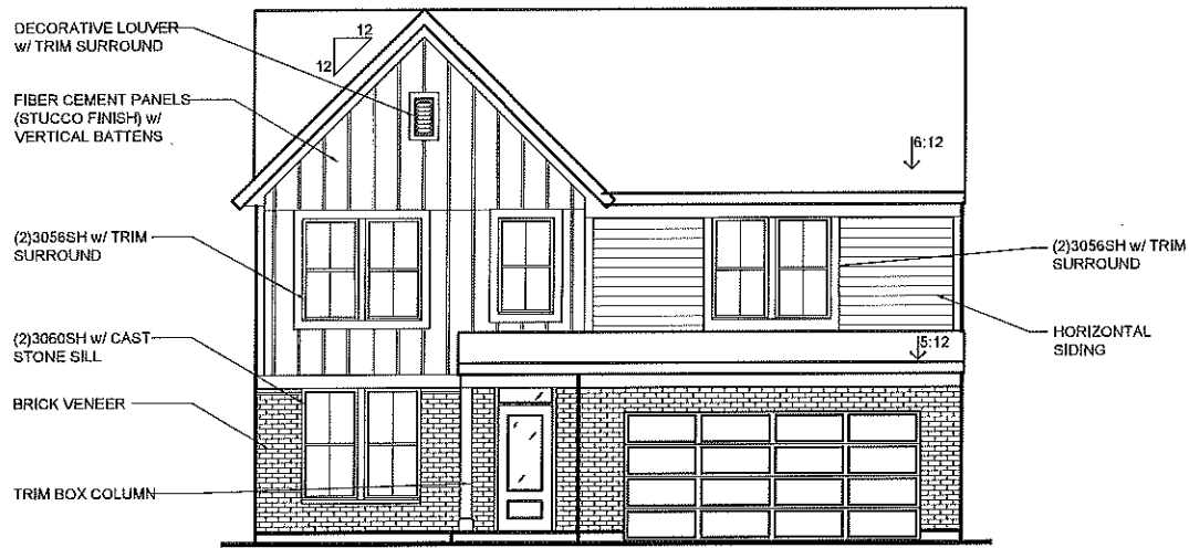
FRONT ENTRY w/ OPT. BRICK VENEER (AVAILABLE w/ LOW or HIGH BRICK SIDES AND REAR)
