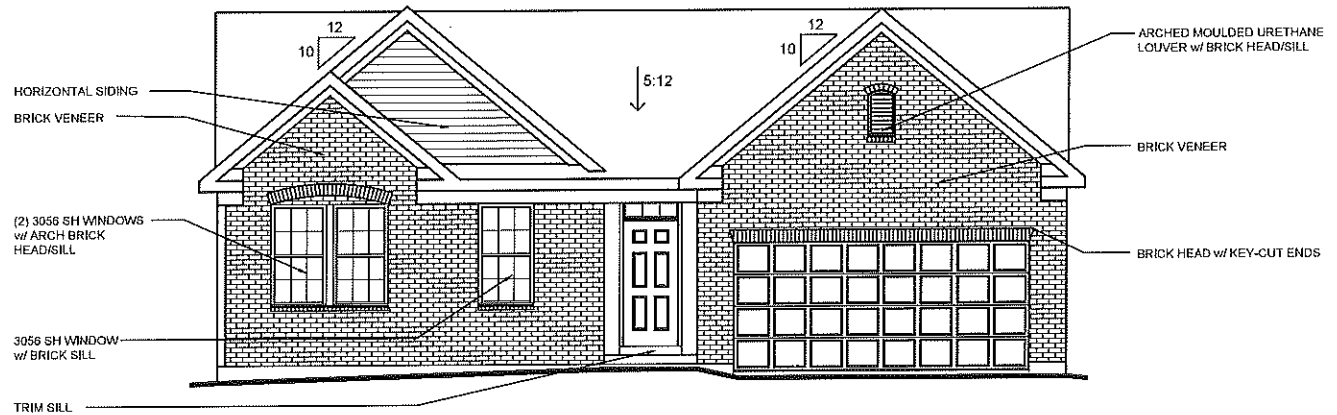
AMERICAN CLASSIC SHOWN W/ OPT. BRICK VENEER (AVAILABLE w/ LOW OR HIGH BRICK SIDES)
