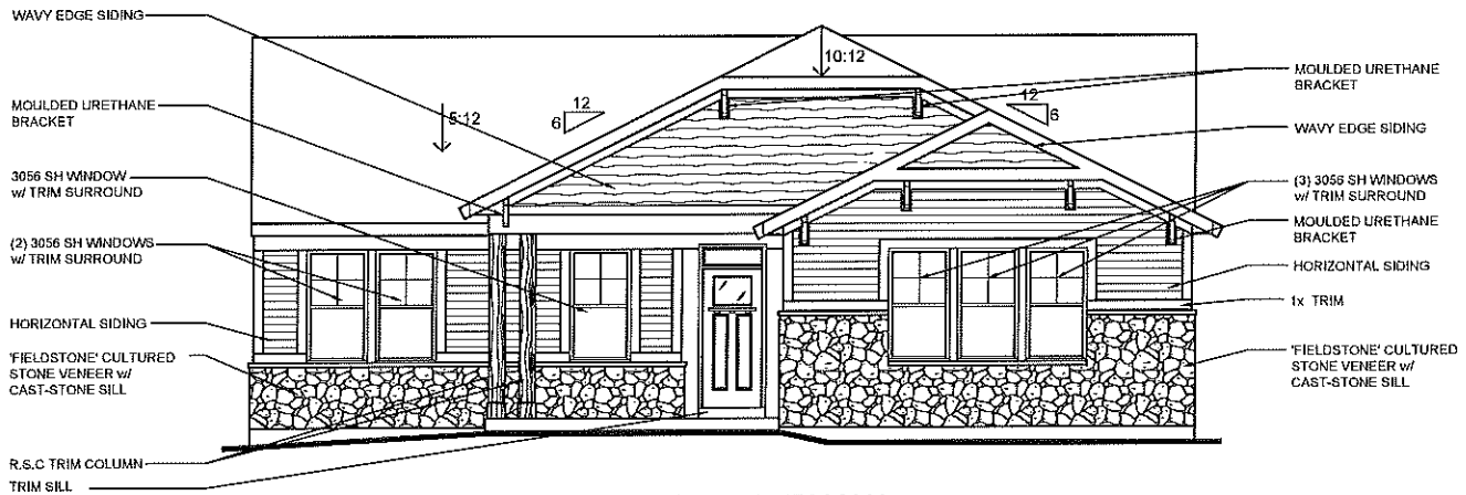
HILLSTONE CRAFTSMAN (SHOWN w/ OPTIONAL SIDE ENTRY GARAGE) SHOWN W/ CULTURED STONE VENEER (AVAILABLE w/ LOW STONE SIDES)
