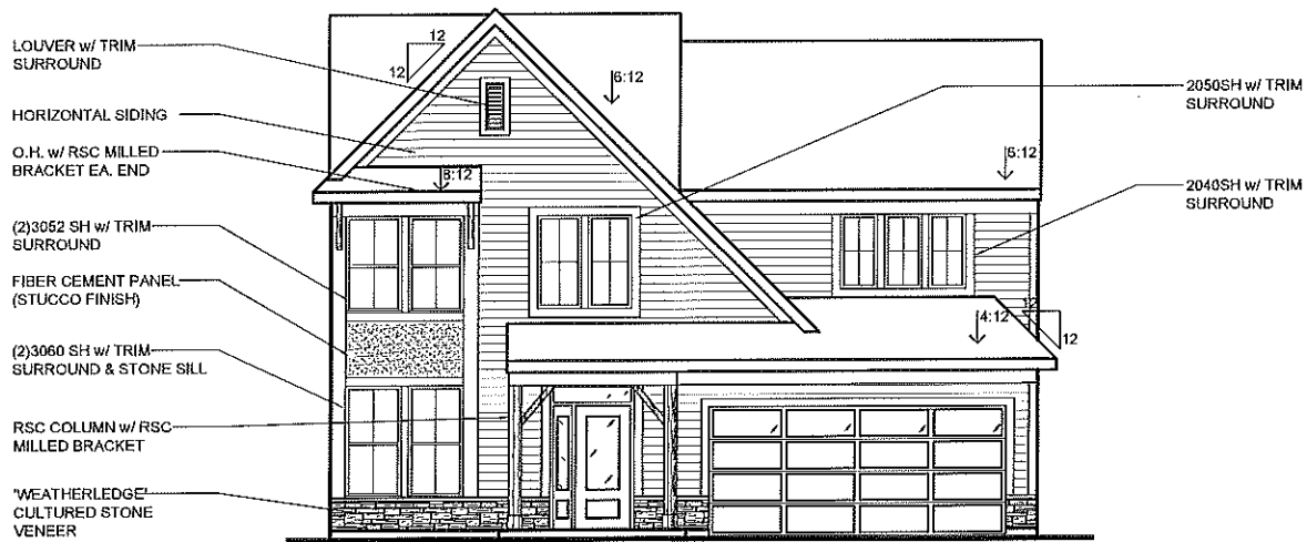
FRONT ENTRY w/ OPT. CULTURED STONE VENEER (AVAILABLE w/ LOW STONE SIDES AND REAR)
