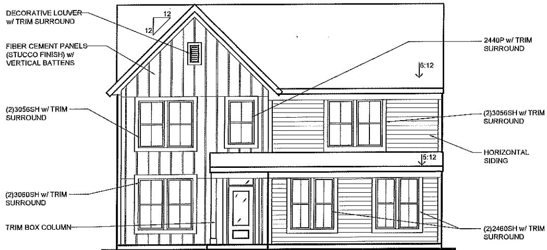
OPT. SIDE ENTRY w/ INCLUDED SIDING
